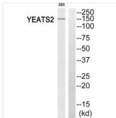
Western blot analysis of extracts from 293 cells, using YEATS2 antibody.
