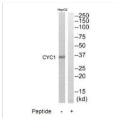
Western blot analysis of extracts from HepG2 cells, using CYC1 antibody.
