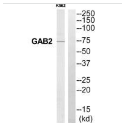
Western blot analysis of extracts from K562 cells, using GAB2 antibody.
