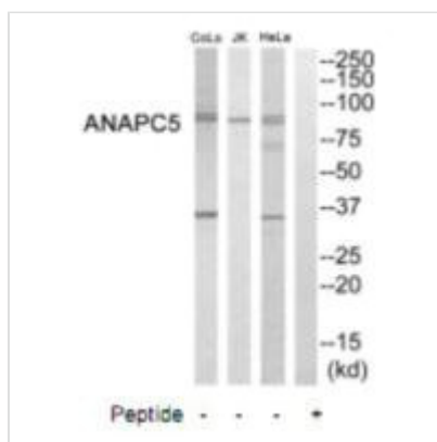
Western blot analysis of extracts from HeLa cells, Jurkat cells and COLO205 cells, using ANAPC5 antibody.
