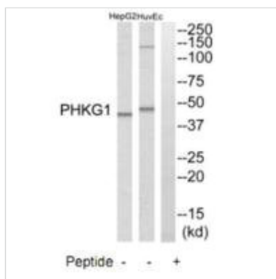
Western blot analysis of extracts from HuvEc cells and HepG2 cells, using PHKG1 antibody.
