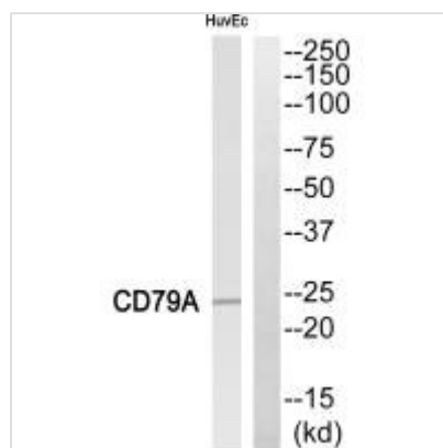
Western blot analysis of extracts from HuvEc cells, using CD79A antibody.
