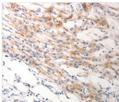
Immunohistochemical analysis of paraffin-embedded Human lung cancer tissue using.
