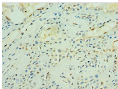
Immunohistochemistry of paraffin-embedded human breast cancer using CSB-PA013505ESR2HU at dilution of 1:100
