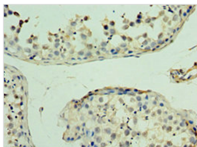
Immunohistochemistry of paraffin-embedded human testis tissue using CSB-PA013505ESR2HU at dilution of 1:100
