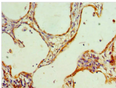
Immunohistochemistry of paraffin-embedded human cervical cancer using CSB-PA010576DSR2HU at dilution of 1:100
