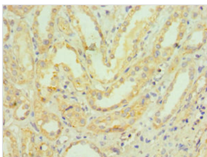
Immunohistochemistry of paraffin-embedded human kidney tissue using CSB-PA010576DSR2HU at dilution of 1:100
