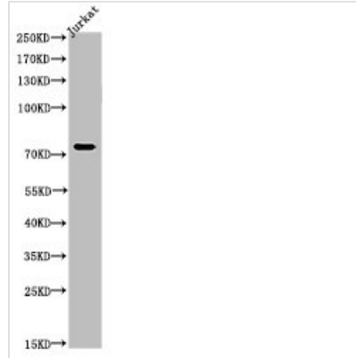
Western Blot analysis of Jurkat cells using Acetyl-p73 (K327) Polyclonal Antibody
