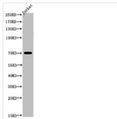
Western Blot analysis of JK cells using Acetyl-p73 (K327) Polyclonal Antibody
