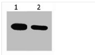
Western blot analysis of CBP recombinant protein, diluted at 1) 1:5000 2) 1:10000
