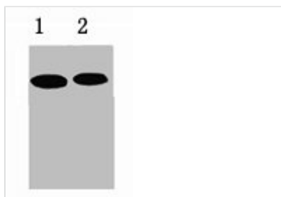
Western blot analysis of GFP Recombinant protein, diluted at 1) 1:5000 2) 1:10000
