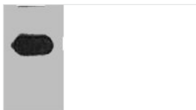
Western blot analysis of mOrange recombinant protein, diluted at 1:5000.
