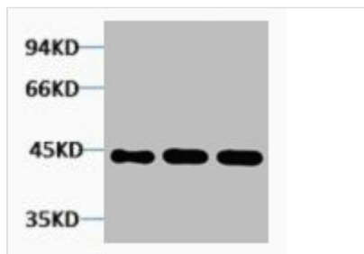
Western blot analysis of 1) HeLa, 2) 3T3, 3) Rat Kidney tissue, diluted at 1:5000.
