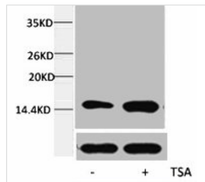
Western blot analysis of extracts from HeLa cells, untreated (-) or treated, 1:5000.
