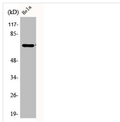
Western Blot analysis of HeLa cells using Phospho-Paxillin (Y31) Polyclonal Antibody
