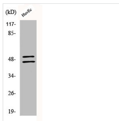
Western Blot analysis of COS7 cells using Phospho-VASP (S157) Polyclonal Antibody
