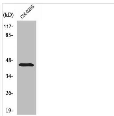
Western Blot analysis of COLO205 cells using ABHD12 Polyclonal Antibody
