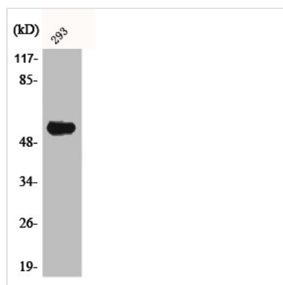
Western Blot analysis of 293 cells using AIRE-1 Polyclonal Antibody
