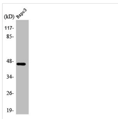
Western Blot analysis of BxPc3 cells using AR-β2 Polyclonal Antibody
