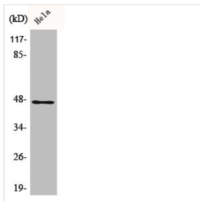
Western Blot analysis of HeLa cells using AW-1 Polyclonal Antibody
