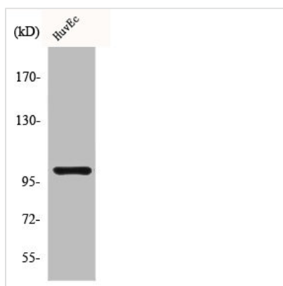
Western Blot analysis of HuvEc cells using Clock Polyclonal Antibody
