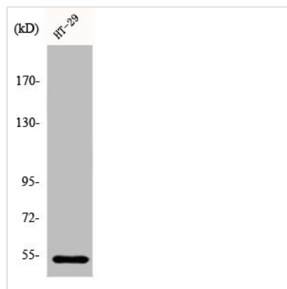
Western Blot analysis of HT29 cells using DDX19B Polyclonal Antibody
