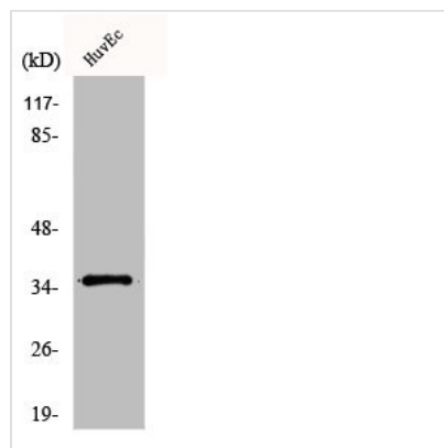
Western Blot analysis of HuvEc cells using DHHC-7 Polyclonal Antibody
