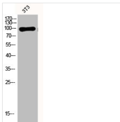
Western Blot analysis of 3T3 cells using Dynamin I Polyclonal Antibody
