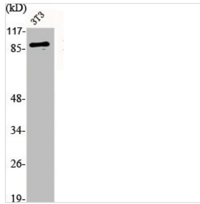
Western Blot analysis of NIH-3T3 cells using Dynamin I Polyclonal Antibody
