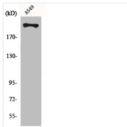
Western Blot analysis of A549 cells using Fatty Acid Synthase Polyclonal Antibody
