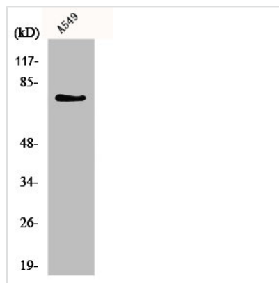
Western Blot analysis of NIH-3T3 cells using GCS- \alpha -1 Polyclonal Antibody
