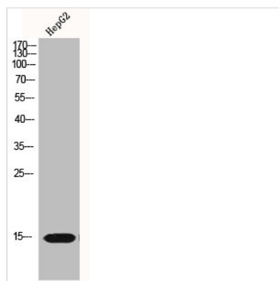
Western Blot analysis of HEPG2 cells using Histone H2A.X Polyclonal Antibody
