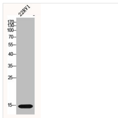
Western Blot analysis of 22RV1 cells using Histone H2A.X Polyclonal Antibody
