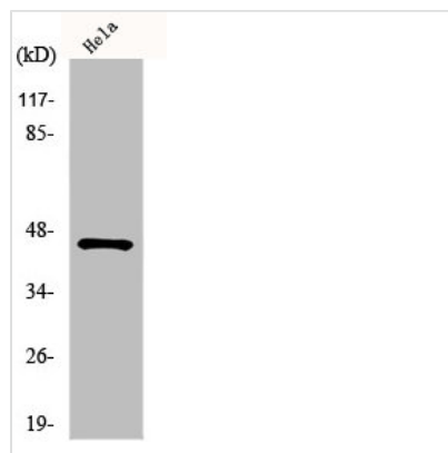
Western Blot analysis of COLO205 cells using HORMAD1 Polyclonal Antibody
