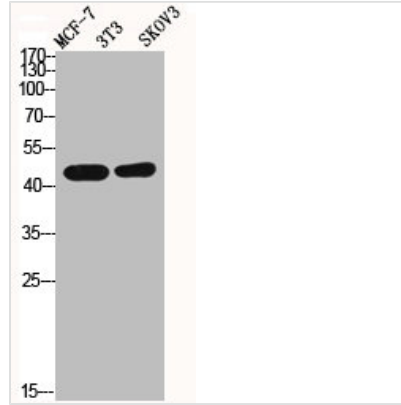
Western Blot analysis of MCF7 NIH-3T3 SKOV3 cells using ICAD Polyclonal Antibody
