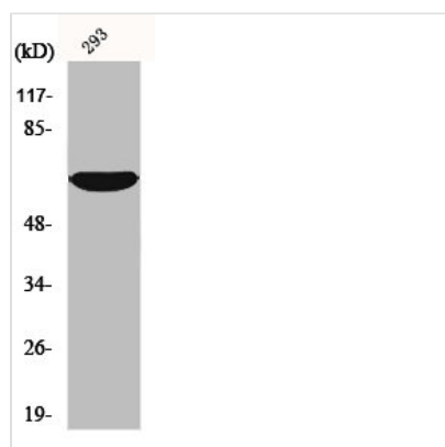
Western Blot analysis of 293 cells using IRAK-2 Polyclonal Antibody
