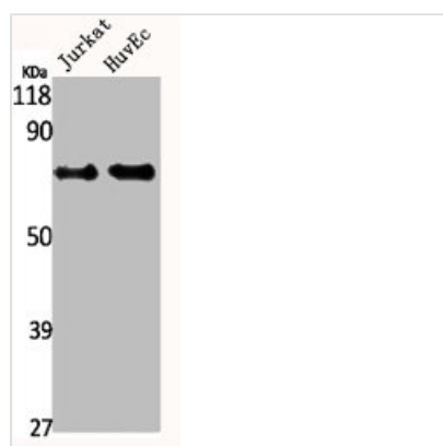
Western Blot analysis of Jurkat HuvEc cells using IRAK-2 Polyclonal Antibody
