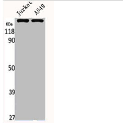
Western Blot analysis of Jurkat A549 cells using MRP7 Polyclonal Antibody
