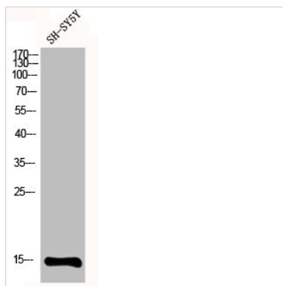
Western Blot analysis of SH-SY5Y cells using MRP-S12 Polyclonal Antibody
