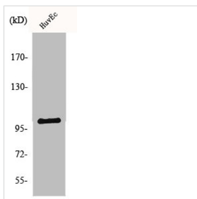
Western Blot analysis of HuvEc cells using NARG1 Polyclonal Antibody
