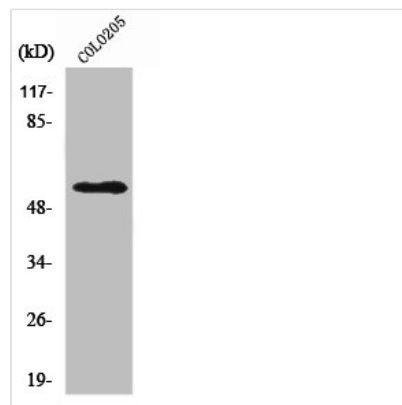
Western Blot analysis of HepG2 cells using NPY5-R Polyclonal Antibody
