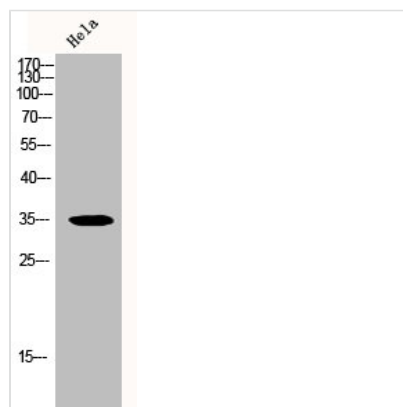
Western Blot analysis of HeLa cells using p53RFP Polyclonal Antibody
