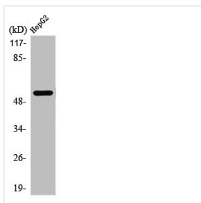
Western Blot analysis of HepG2 cells using PREP-2 Polyclonal Antibody
