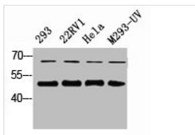
Western Blot analysis of 823 22RV1 HELA 293-UV cells using Smad2/3 Polyclonal Antibody
