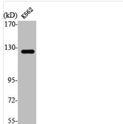
Western Blot analysis of K562 cells using ST5 Polyclonal Antibody
