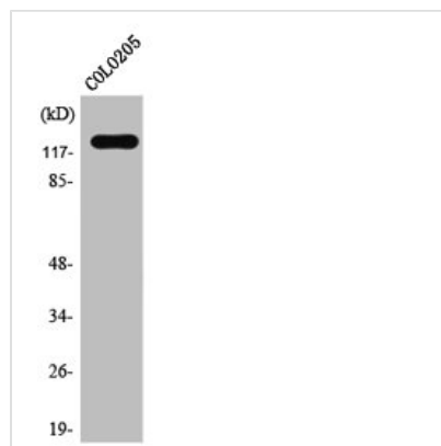
Western Blot analysis of COLO205 cells using ST5 Polyclonal Antibody
