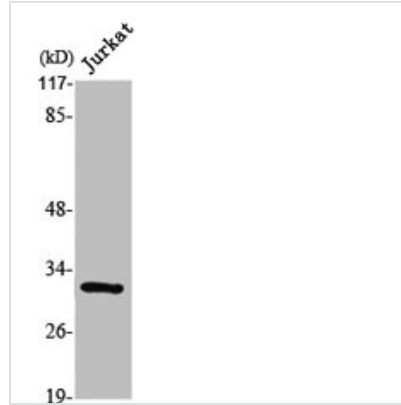
Western Blot analysis of Jurkat cells using SURF-1 Polyclonal Antibody
