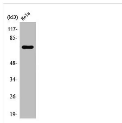
Western Blot analysis of HepG2 cells using TAP Polyclonal Antibody
