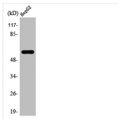
Western Blot analysis of HepG2 cells using TCP-1 ζ Polyclonal Antibody
