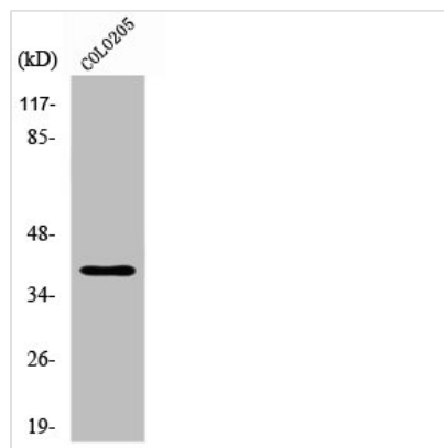
Western Blot analysis of COLO205 cells using XRCC4 Polyclonal Antibody
