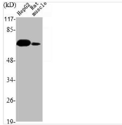
Western Blot analysis of HepG2 RAT-MUSCLE cells using YAP Polyclonal Antibody
