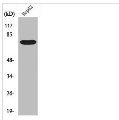
Western Blot analysis of HepG2 cells using YAP Polyclonal Antibody
