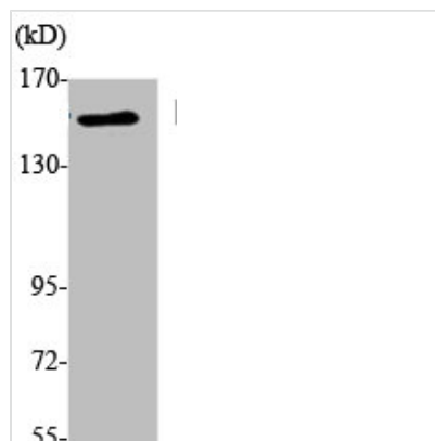
Western Blot analysis of K562 cells using EEA1 Polyclonal Antibody
