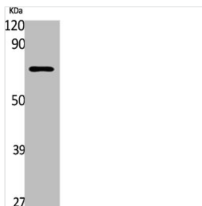
Western Blot analysis of Jurkat cells using GABAA Rε Polyclonal Antibody
