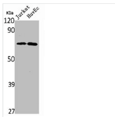
Western Blot analysis of Jurkat HuvEc cells using HNF-1β Polyclonal Antibody
