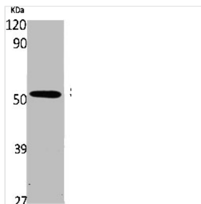
Western Blot analysis of K562 cells using Smad5 Polyclonal Antibody
