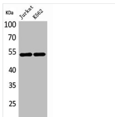
Western Blot analysis of Jurkat K562 cells using HNF-4 \alpha / \gamma Polyclonal Antibody
