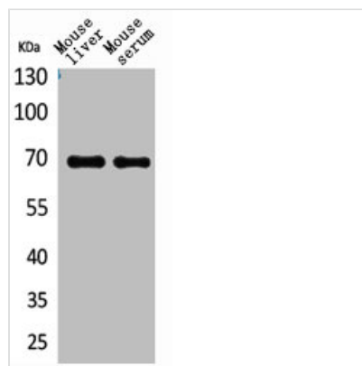
Western Blot analysis of mouse liver mouse serum cells using AFP Polyclonal Antibody
